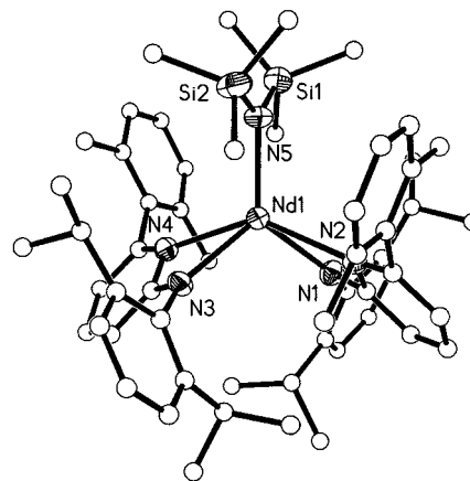
Figure 3. Molecular structure of 7 (ellipsoids correspond to the 50% probability level); selected bond lengths [Å] and angles [°]: Nd1–N5 2.280(2), Nd1–N3 2.407(2), Nd1–N1 2.414(2), Nd1–N2 2.544(2), Nd1–N4 2.552(2); N5–Nd1–N3 123.78(8), N5–Nd1–N1 125.18(8), N5–Nd1–N2 108.02(8), N1–Nd1–N2 54.56(7), N5–Nd1–N4 110.50(8), N3–Nd1–N4 54.57(7).
