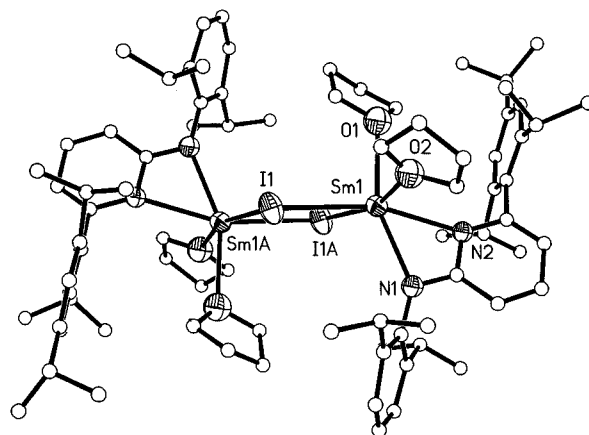
Figure 5. Molecular structure of 9 (ellipsoids correspond to the 50% probability level).
