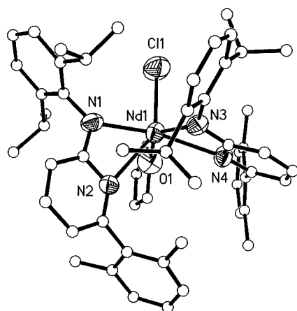
Figure 2. Molecular structure of 6 (ellipsoids correspond to the 50% probability level); selected bond lengths [Å] and angles [°]: Nd1–N1 2.361(6), Nd1–N3 2.386(7), Nd1–O1 2.442(7), Nd1–N4 2.569(6), Nd1–Cl1 2.599(3), Nd1–N2 2.622(6), Nd1–C1 2.936(8), N3–Nd1–N4 54.9(2), N1–Nd1–Cl1 90.50(17), N3–Nd1–Cl1 103.37(16), N4–Nd1–Cl1 107.91(15), N1–Nd1–N2 54.1(2), Cl1–Nd1–N2 142.91(14).
