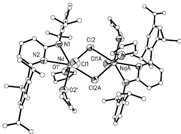
Figure 1. Molecular structure of 5 (ellipsoids correspond to the 50% probability level); selected bond lengths [Å] and angles [°]: Nd–N1 2.380(4), Nd–O2' 2.510(4), Nd–O1' 2.510(4), Nd–Cl1 2.6443(19), Nd–N2 2.659(4), Nd–Cl2 2.7919(17), Nd–Cl2A 2.8511(17); Nd–Cl2–NdA 108.37(5), Cl1–Nd–Cl2 99.81(6), N1–Nd–N2 53.25(14).
