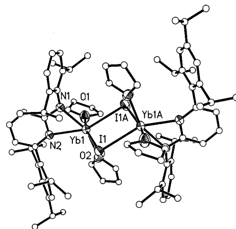
Figure 4. Molecular structure of 8 (ellipsoids correspond to the 50% probability level); selected bond lengths [Å] and angles [ ^\circ ]: \text{Yb1-N1} 2.423(4), \text{Yb1-O2} 2.432(4), \text{Yb1-O1} 2.445(4), \text{Yb1-N2} 2.508(4), \text{Yb1-C1} 2.922(5), \text{Yb1-I1} 3.1225(10), \text{Yb1-I1} 3.1241(8), \text{I1-Yb1} 3.1225(10); \text{N1-Yb1-O1} 156.82(14), \text{N1-Yb1-O2} 97.23(15), \text{O2-Yb1-O1} 81.22(15), \text{N1-Yb1-N2} 55.30(13), \text{O2-Yb1-N2} 101.54(13), \text{O1-Yb1-N2} 87.55(14), \text{N1-Yb1-I1A} 104.44(10), \text{O2-Yb1-I1A} 98.42(10), \text{O1-Yb1-I1A} 83.99(11), \text{N2-Yb1-I1A} 156.84(9), \text{N1-Yb1-I1} 97.46(10), \text{O2-Yb1-I1} 87.29(10), \text{O1-Yb1-I1} 164.43(10), \text{N2-Yb1-I1} 105.12(9), \text{C1-Yb1-I1} 102.77(9), \text{I1-Yb1-I1A} 87.36(3).
