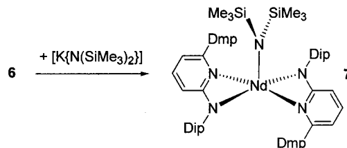
Scheme 6. Synthesis of 7 .
